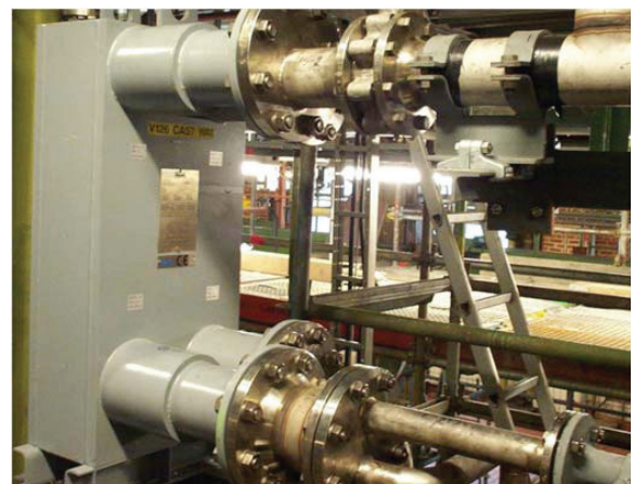
SIGMAWIG ST30 for steam condensation
